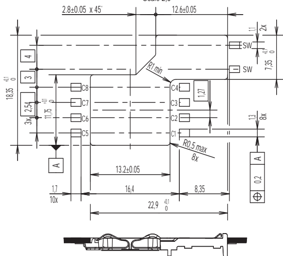
RECOMMENDED PC BOARD LAYOUT (Component side)
