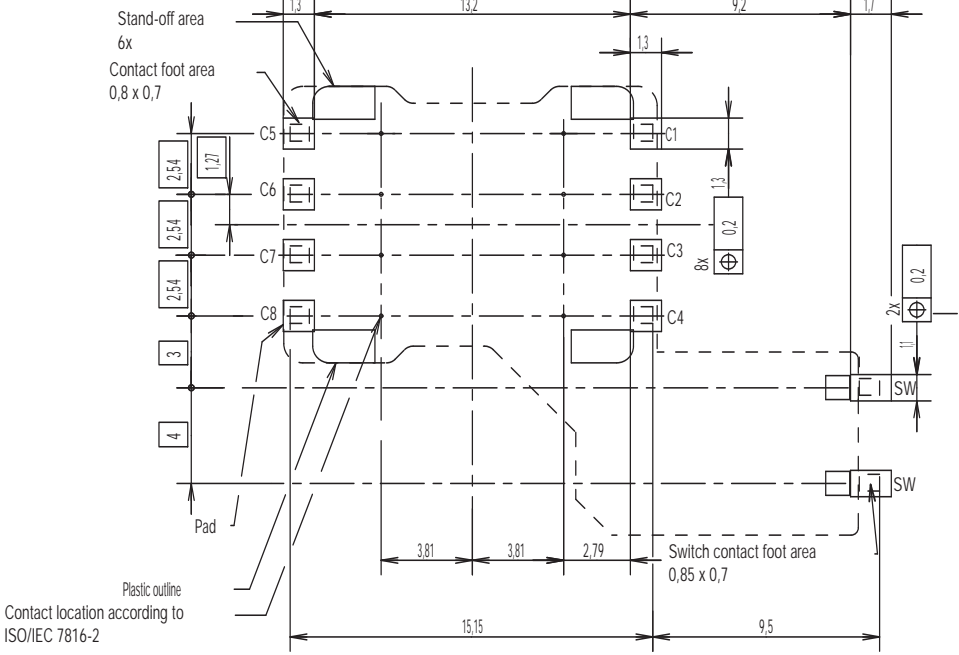
RECOMMENDED PC BOARD LAYOUT (Component side)
