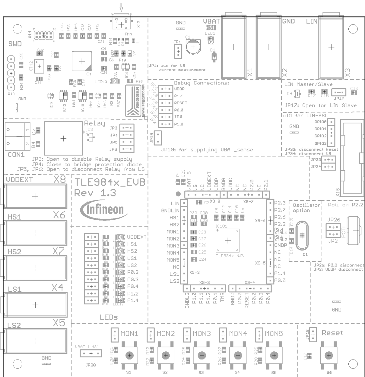
Figure 8 Parts placement
