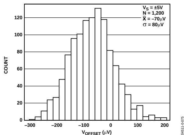
Figure 52. Input Offset Voltage Distribution
