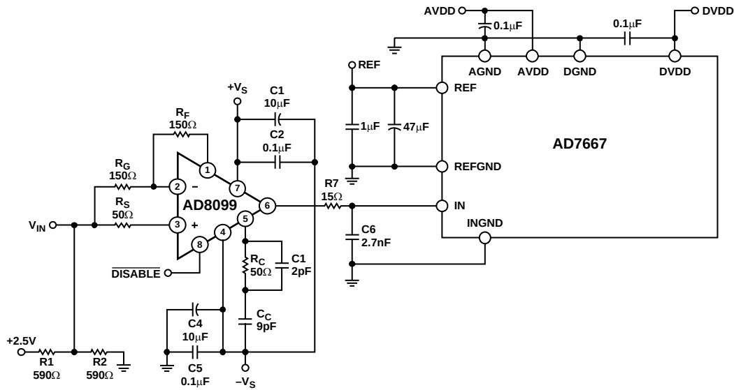
Figure 76. ADC Driver
