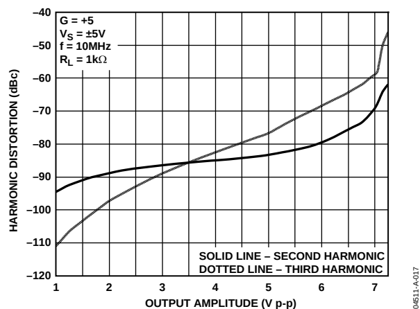
Figure 31. Harmonic Distortion vs. Output Amplitude (SOIC)
