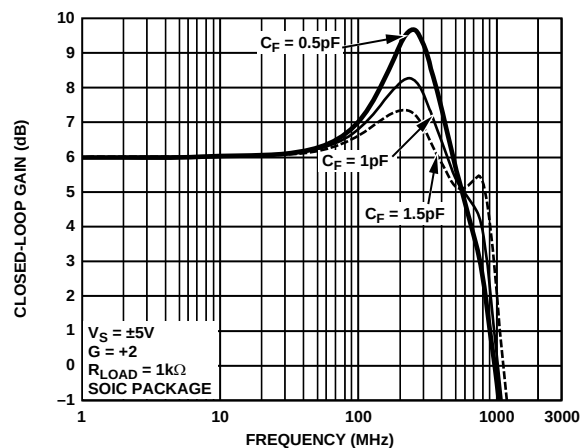
Figure 71. Frequency Response for Various Values of C_F
