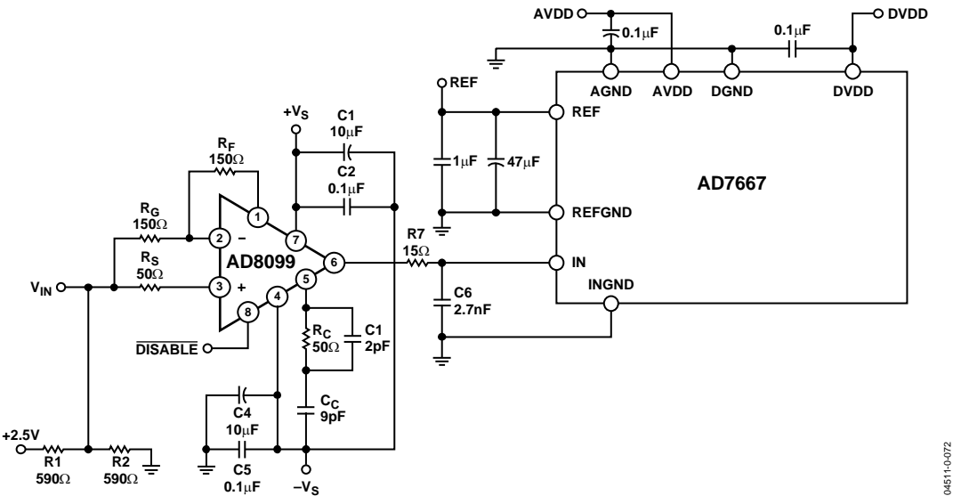
Figure 76. ADC Driver
