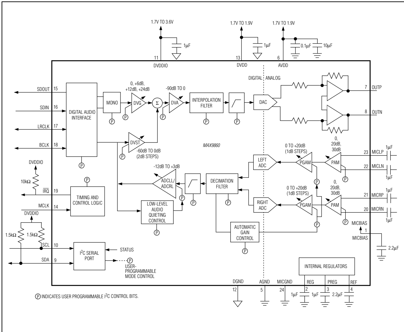
Functional Diagram/Typical Operating Circuit
