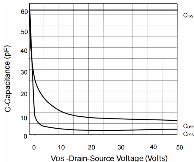
Capacitance v drain-source voltage
