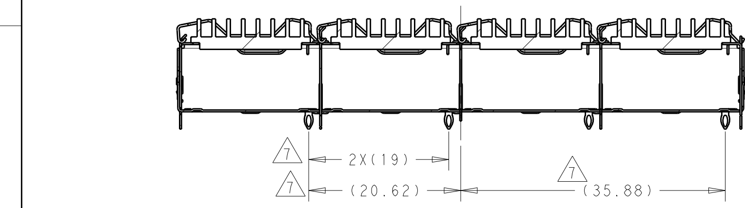
For 2343988-1/-2-3 WITH REAR EONS SECTION W-W
