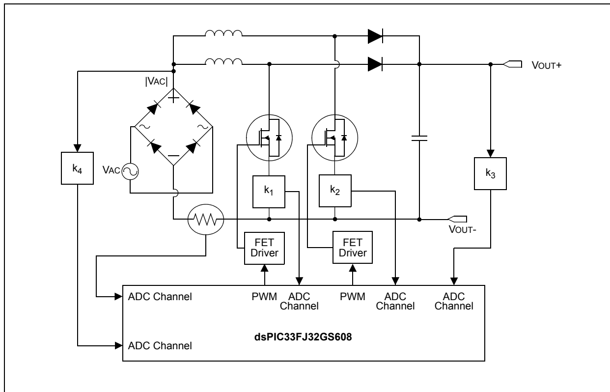
FIGURE 2-9: INTERLEAVED PFC
