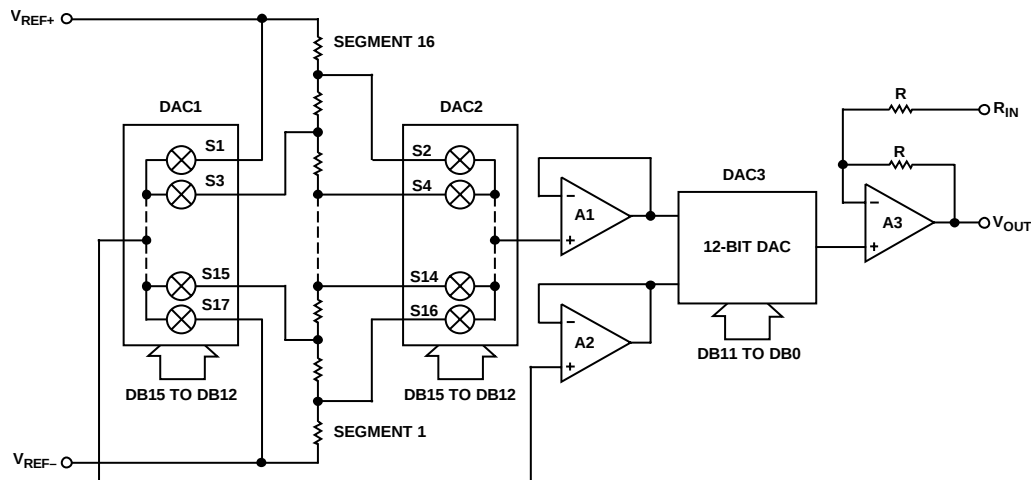
Figure 21. Digital-to-Analog Conversion
