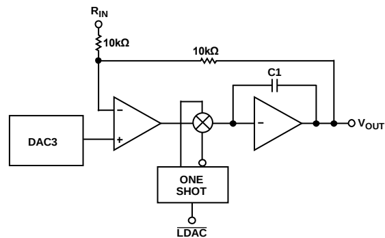
Figure 22. Output Stage
