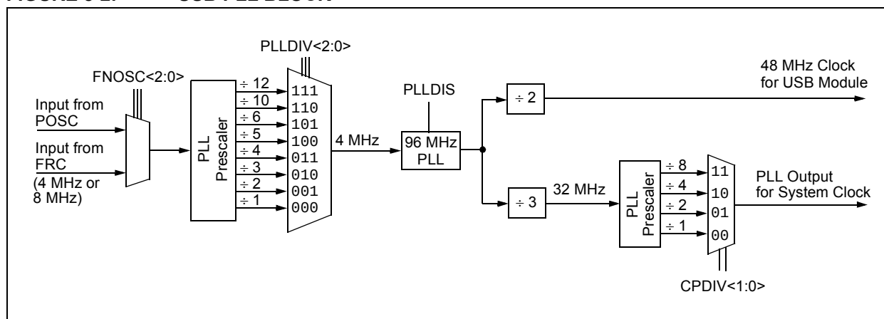
FIGURE 8-2: USB PLL BLOCK
