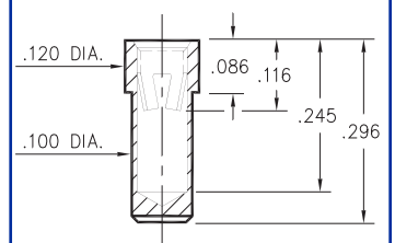
8829-0-15-XX-23-XX-10-0 Solder mount in .102 min. mounting hole
