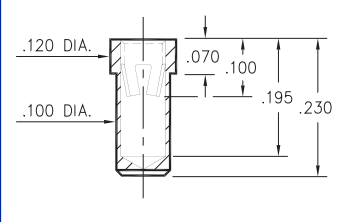
9801-0-15-XX-23-XX-10-0 Solder mount in .102 min. mounting hole Also available on 16mm wide carrier tape: 1,200 parts per 13" reel. Order as: 9801-0-57-XX-23-XX-10-0
