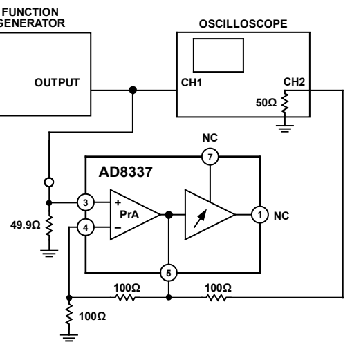
Figure 55. Preamp Overdrive Recovery
