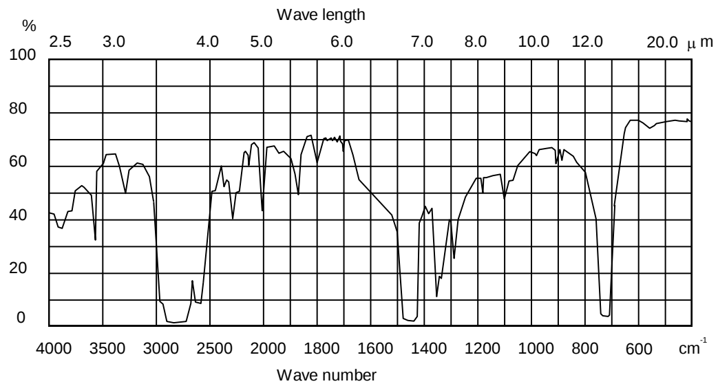
Figure 4. Transmittance
