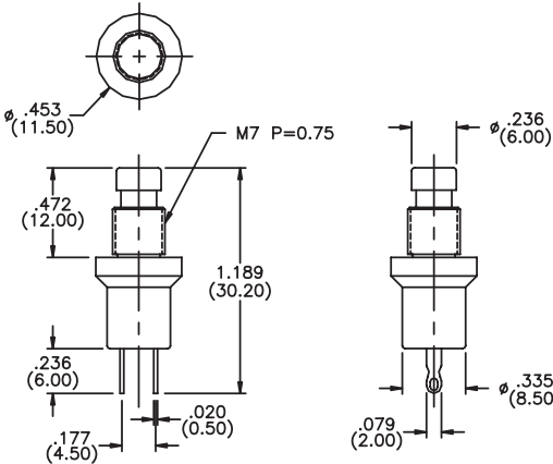
MECHANICAL OUTLINE
