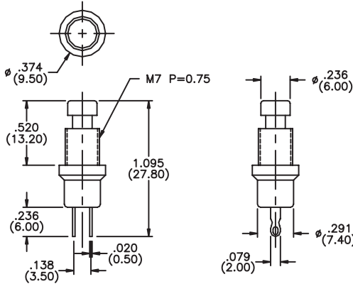
MECHANICAL OUTLINE
