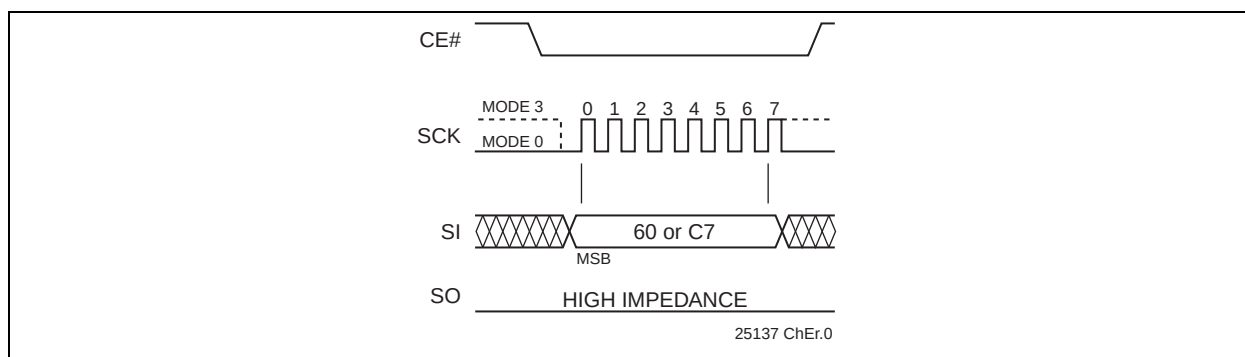
FIGURE 4-13: CHIP-ERASE SEQUENCE
