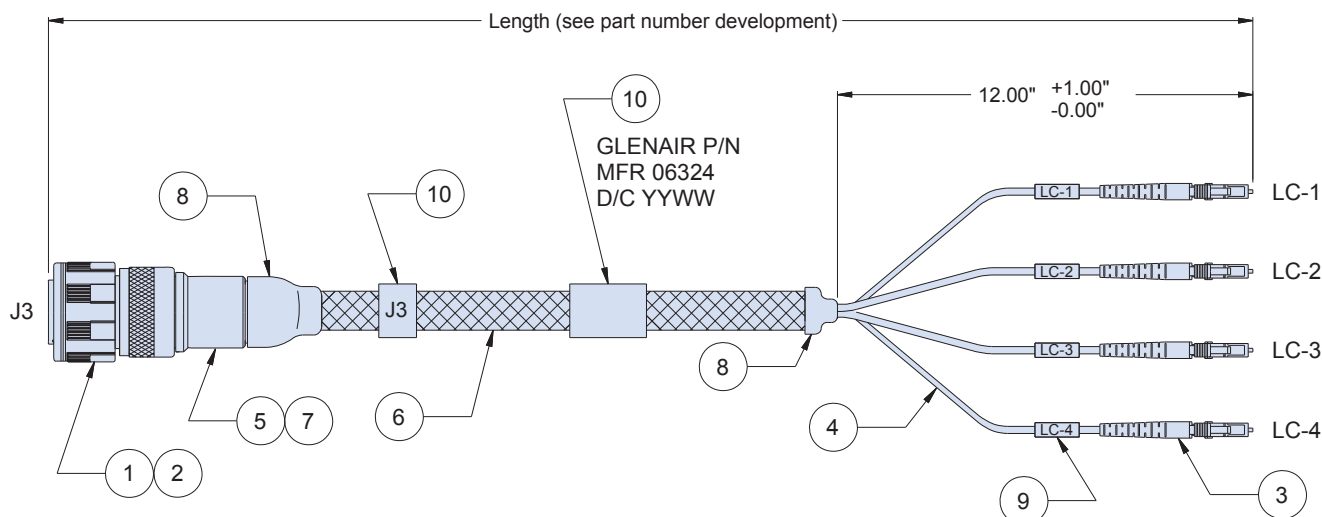
Connection Diagram
