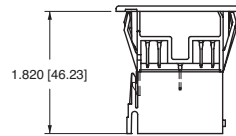
VHP CONTURA II, III HOLE PLUG (With VC1 connector attached)
