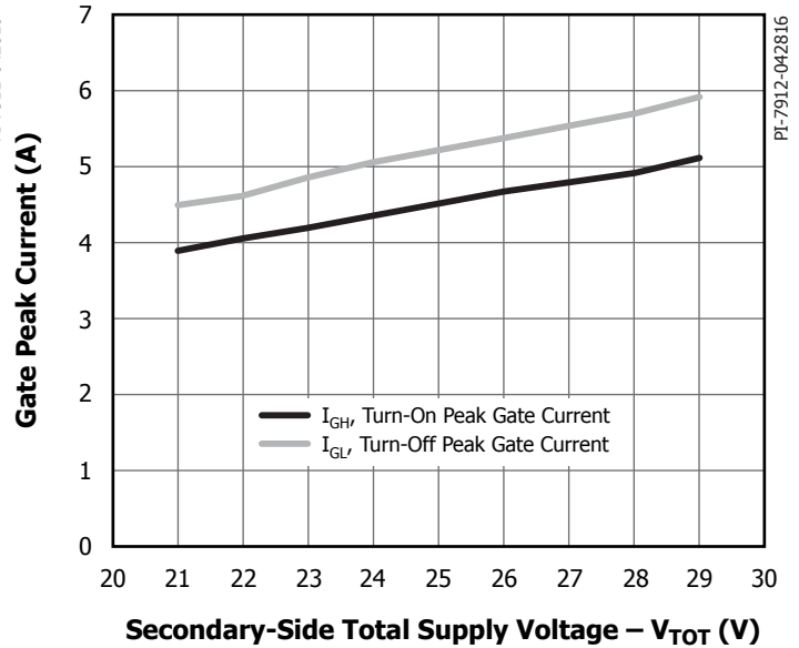
Figure 8. Turn-On and Turn-Off Peak Output Current vs. Secondary-Side Total Supply Voltage ( V_{TOT} ). Conditions: V_{CC} = 5 \text{ V} , T_j = 25 \text{ °C} , R_{GH} = 4 \Omega , R_{GL} = 3.4 \Omega , C_{LOAD} = 100 \text{ nF} , f_s = 1 \text{ kHz} , Duty Cycle = 50%.
