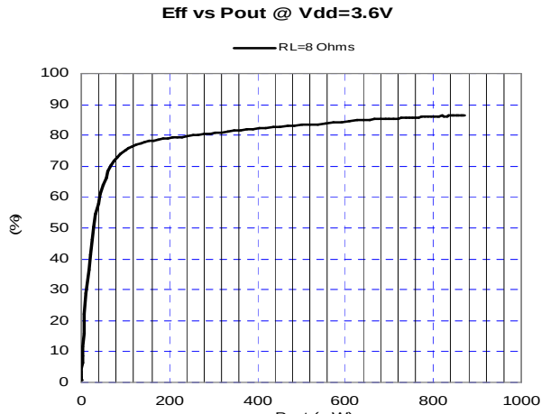
Figure 4. Efficiency vs. P_{OUT} , R_L=8\ \Omega , f=1\text{kHz}
