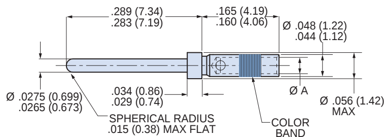
#23 Pin Contact
