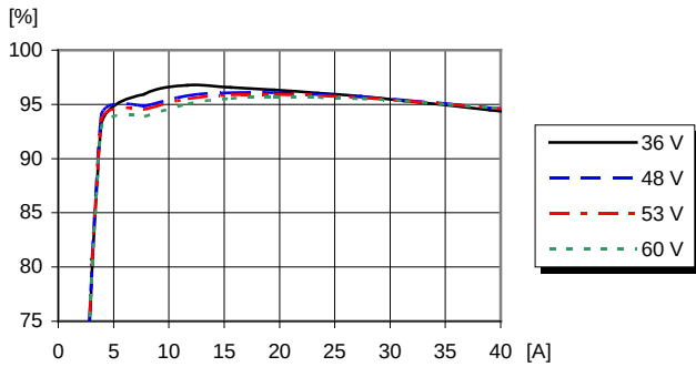
Efficiency vs. load current and input voltage at T_{P1}, T_{P3} = +25^{\circ}\text{C}
