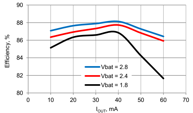
Figure 11-9. Efficiency vs I OUT V BOOST = 3.3 V, L BOOST = 22 \mu H [29]
