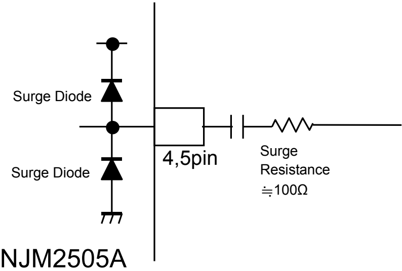
Fig1: External connection
