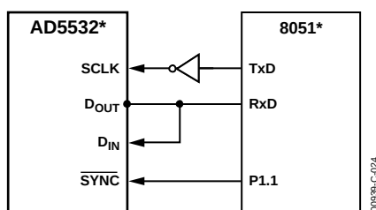
Figure 25. AD5532 to 8051 Interface
