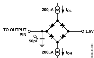
Figure 3. Load Circuit for D_{\text{OUT}} Timing Specifications
