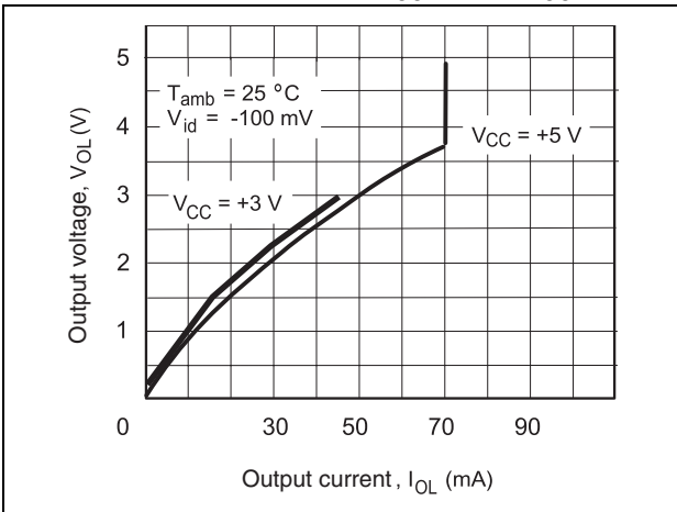
Figure 4. Low level output voltage vs. low level output current ( V_{CC} = +5\text{ V} , V_{CC} = +3\text{ V} )
