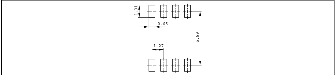
Figure 31 Footprint PG-DSO-8
