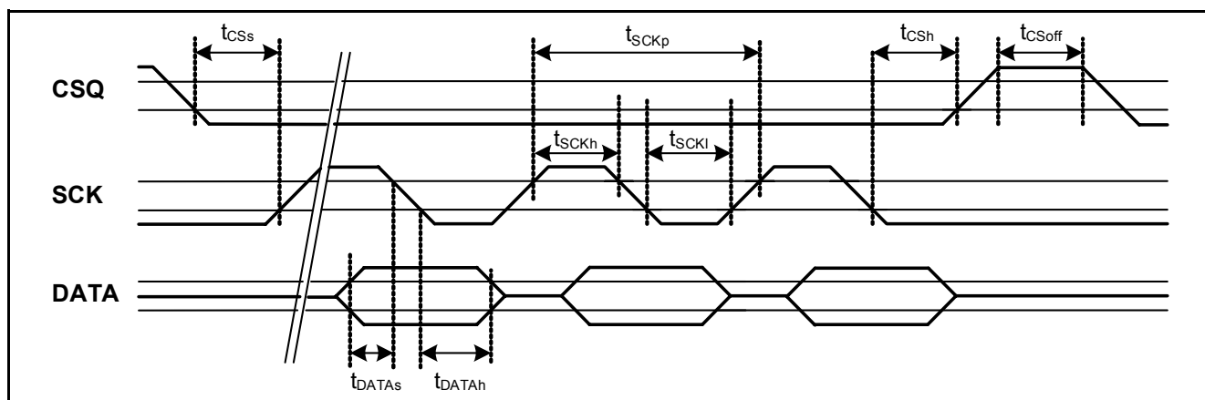
Figure 16 SSC Timing
