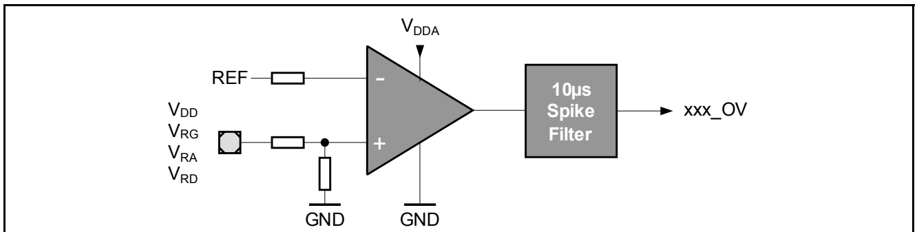
Figure 27 OV Comparator
