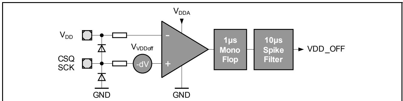
Figure 29 V_{DD} - Off Comparator
