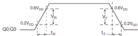
OUTPUT RISE/FALL SLEW RATES
