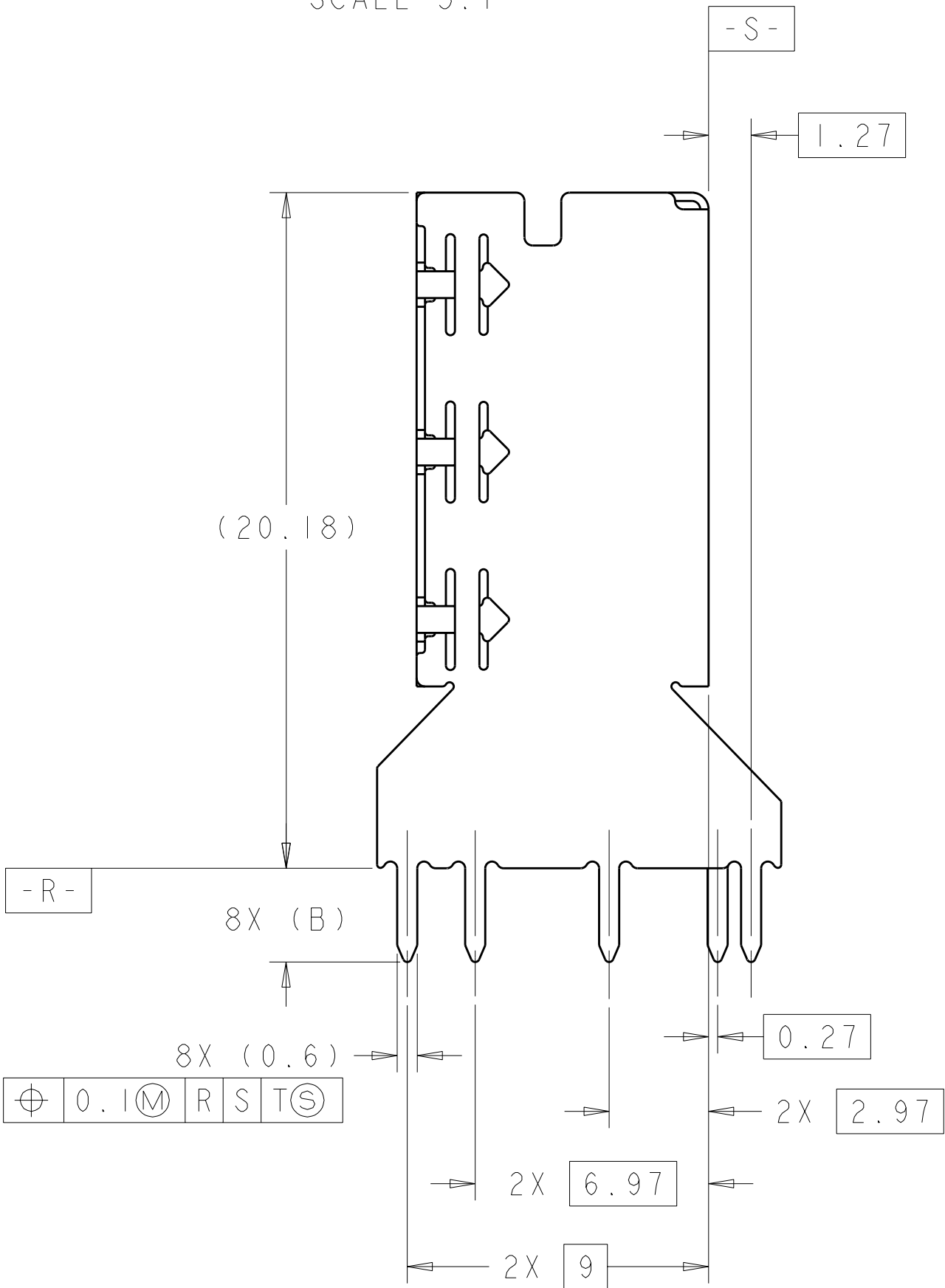
1888413-6 SCALE 5:1
