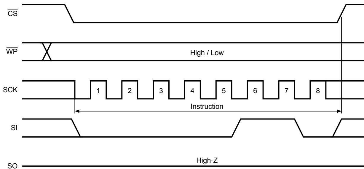
Figure 11 WREN Operation
