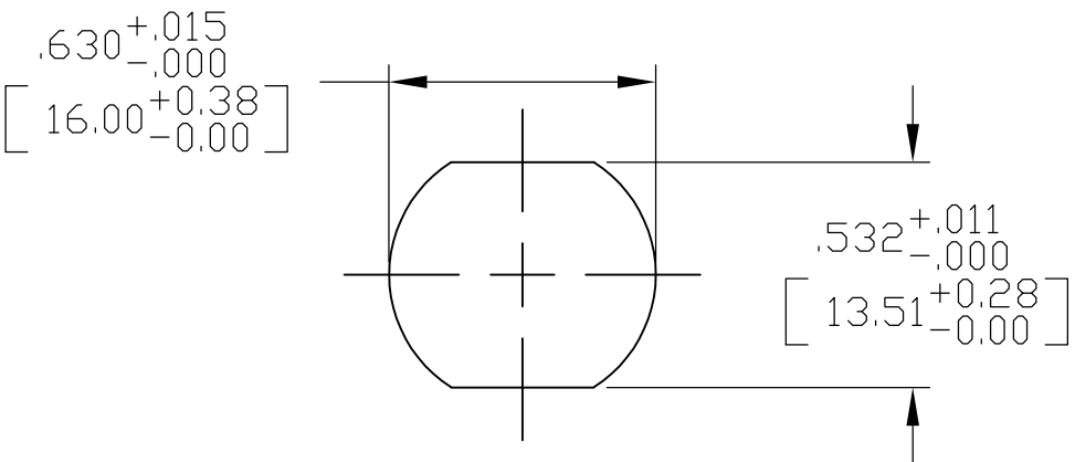
RECOMMENDED PANEL CUTOUT SCALE 2:1
