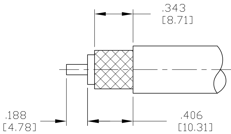
RECOMMENDED STRIP LENGTH SCALE 2:1
