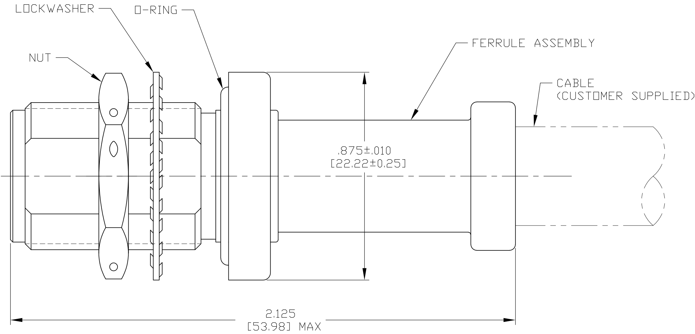
ASSEMBLED VIEW
