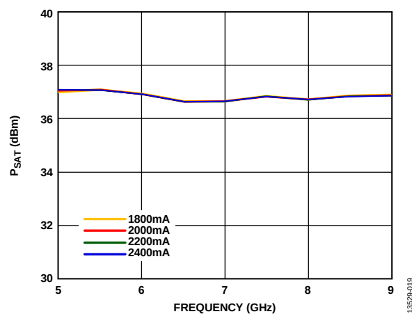
Figure 19. P_{SAT} vs. Frequency at Various Supply Currents ( I_{DD} )
