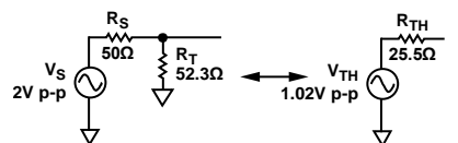
Figure 68. Calculating the Thevenin Equivalent
