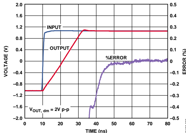
Figure 46. 0.1% Settling Time
