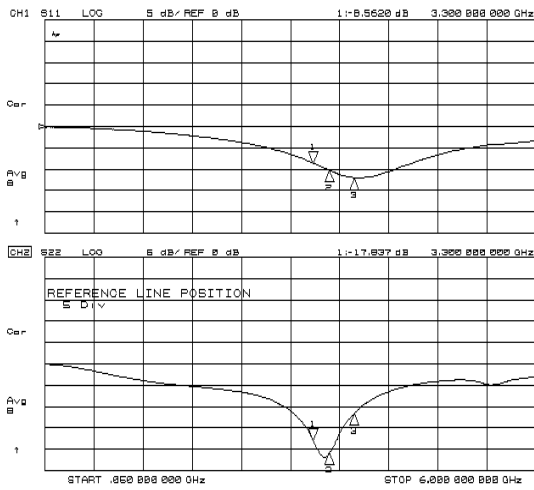
S11, S22
