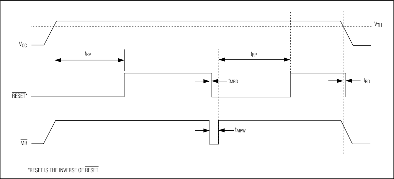
Figure 2. \text{RESET}^* Timing Relationship
