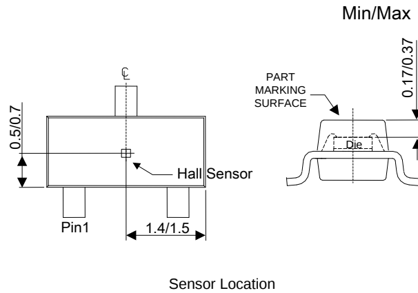
Sensor Location
