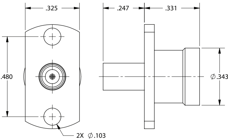
SMP Male LD to ZMA Female, Thread-In
