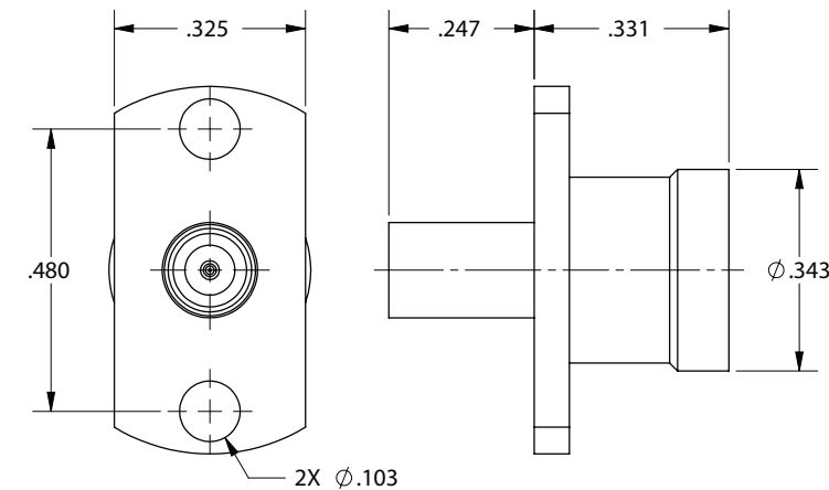
SMP Male LD to ZMA Female, Thread-In
