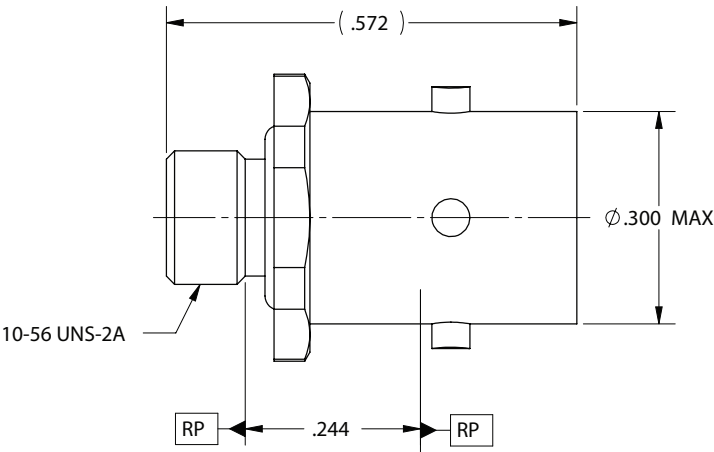
SMP Male LD to ZMA Female, Thread-In
