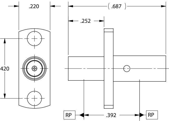
SMP Male to SVMS Male SB, Two Hole Flange Mount
