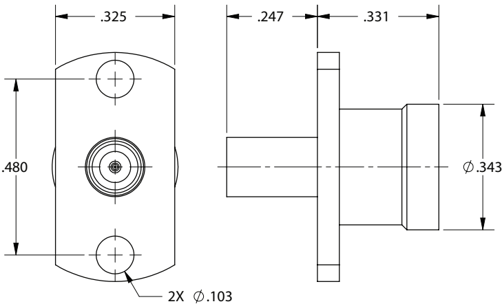
SMP Male LD to ZMA Female, Thread-In
