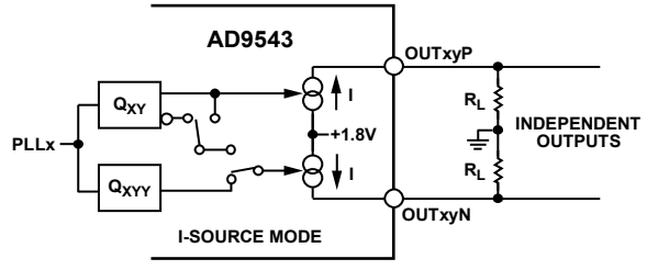
Figure 38. Dual-Divider, Single-Ended Mode Providing Independent Outputs (Current Source Mode); Note that Single-Ended CML Mode is Also Available (See Figure 33)
