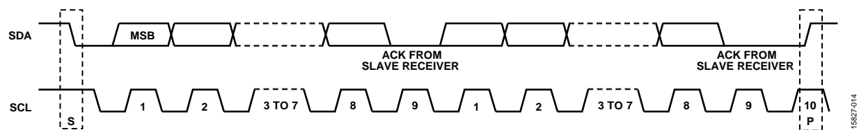
Figure 62. Acknowledge Bit
