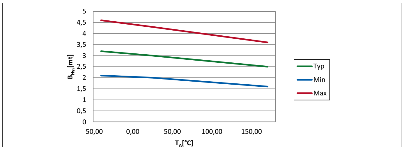
Figure 5-3 Hysteresis ( B_{Hys} ) of the TLE4964-3K over Temperature
