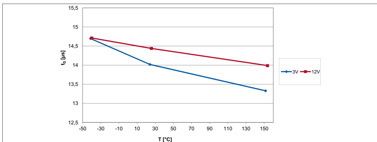
Figure 6-2 Signal Delay Time of the TLE4964-3K over Temperature
