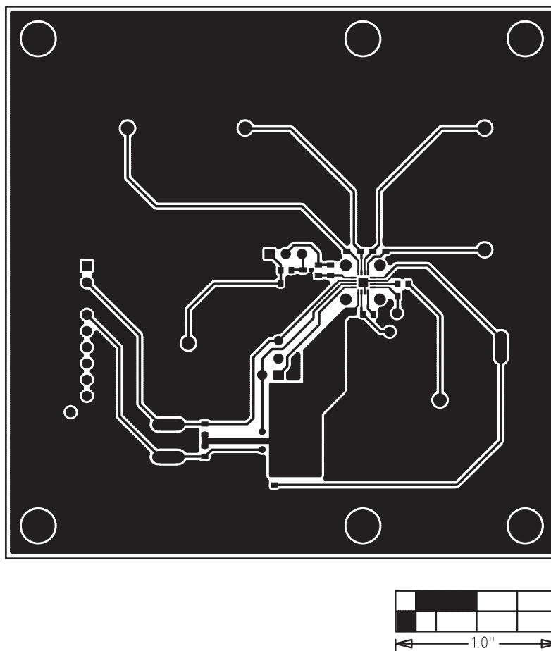
Figure 5. MAX9507 EV Kit PCB Layout—Component Side
