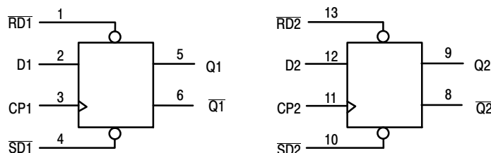
Figure 1. LOGIC DIAGRAM
