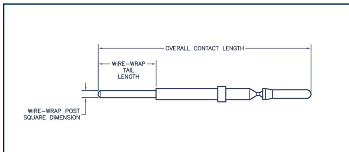
Wire-Wrap Contact
