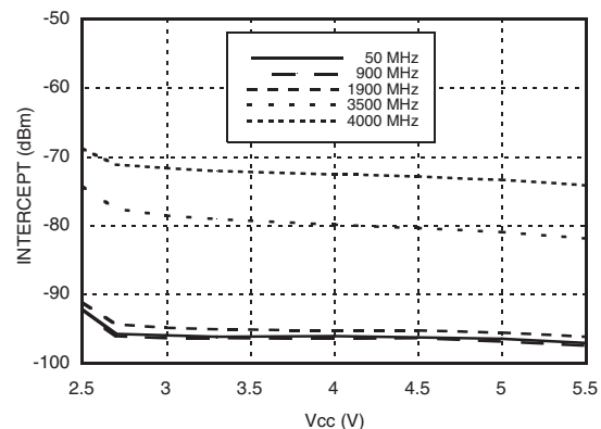
LOGOUT Intercept vs. Bias Voltage T A = +25°C
