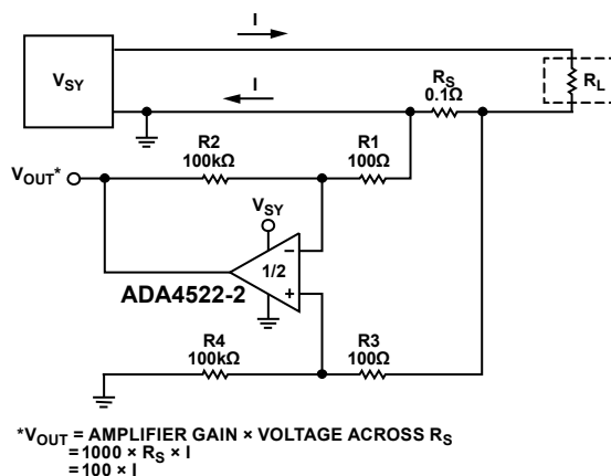
Figure 81. Low-Side Current Sensing
