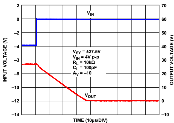
Figure 54. Positive Overload Recovery, V_{SY} = \pm 27.5V
