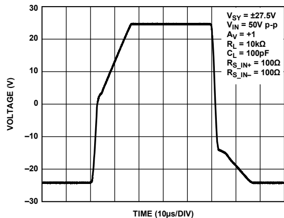
Figure 36. Large Signal Transient Response, V_{SY} = \pm 27.5V
