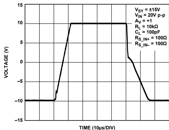
Figure 35. Large Signal Transient Response, V_{SY} = \pm 15V
