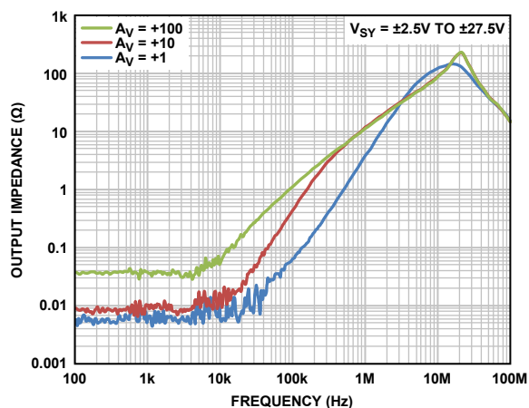
Figure 29. Closed-Loop Output Impedance vs. Frequency
