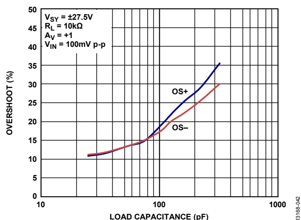
Figure 42. Small Signal Overshoot vs. Load Capacitance, V_{SY} = \pm 27.5 V
