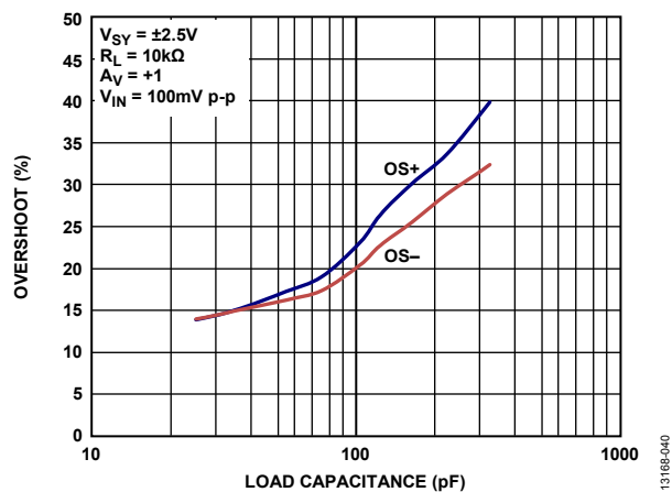
Figure 40. Small Signal Overshoot vs. Load Capacitance, V_{SY} = \pm 2.5 V
