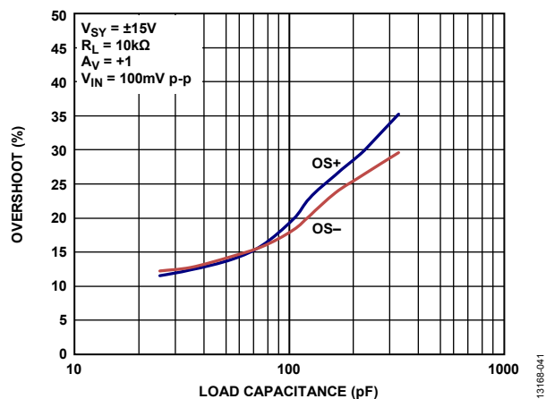
Figure 41. Small Signal Overshoot vs. Load Capacitance, V_{SY} = \pm 15 V
