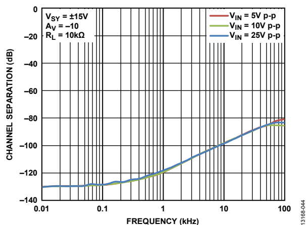
Figure 44. Channel Separation vs. Frequency, V_{SY} = \pm 15 V
