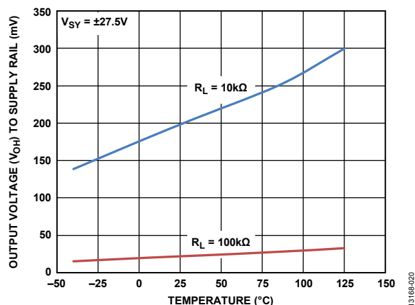
Figure 24. Output Voltage High ( V_{OH} ) to Supply Rail vs. Temperature, V_{SY} = \pm 27.5\text{V}
