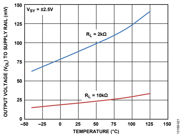
Figure 25. Output Voltage Low ( V_{OL} ) to Supply Rail vs. Temperature, V_{SY} = \pm 2.5\text{V}
