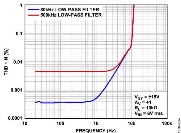
Figure 50. THD + N vs. Frequency, V_{SY} = \pm 15V
