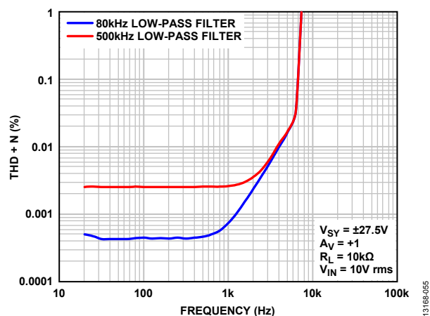
Figure 51. THD + N vs. Frequency, V_{SY} = \pm 27.5V
