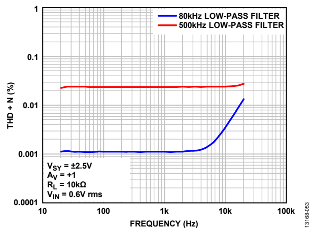
Figure 49. THD + N vs. Frequency, V_{SY} = \pm 2.5V
